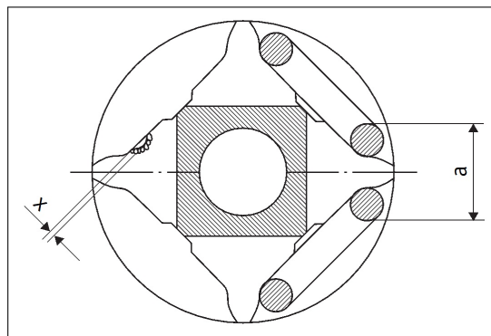
Figure 16: Four-tooth chain sprocket
